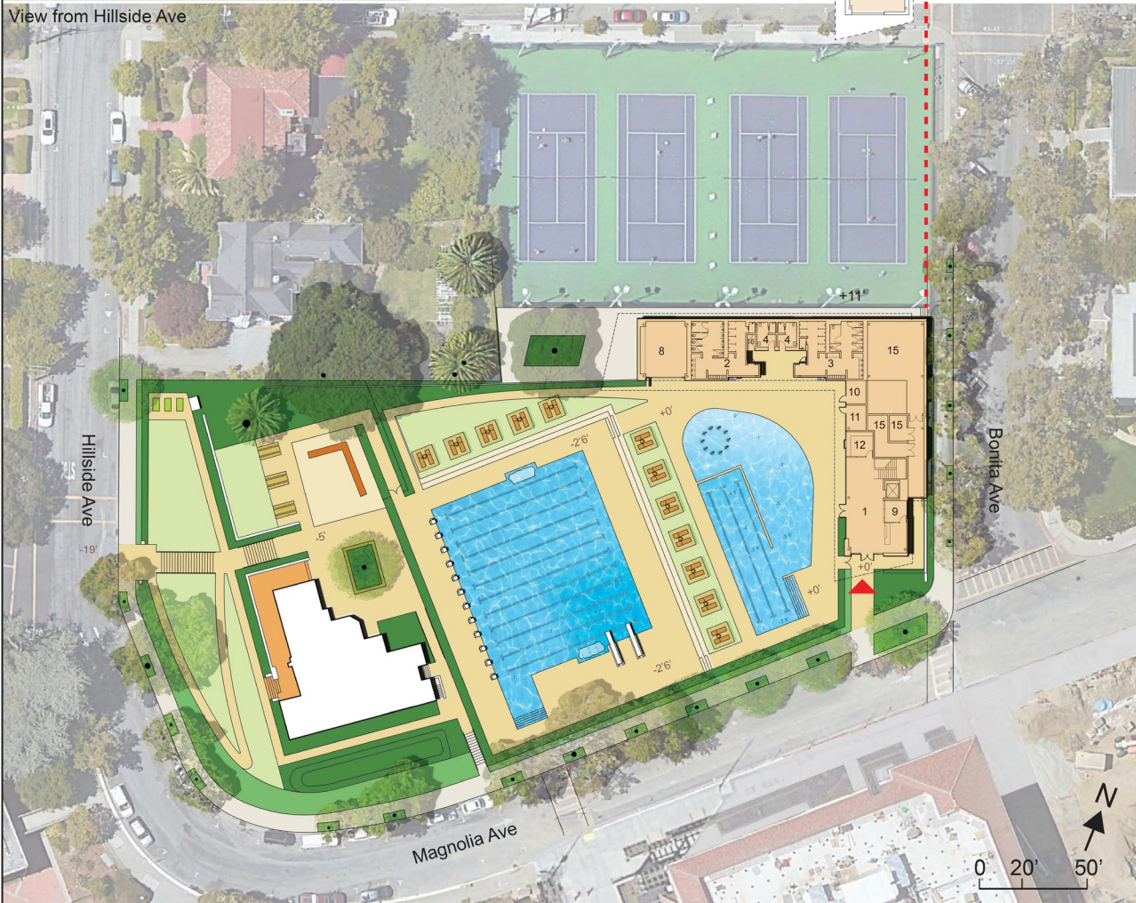
Site Plan / First Floor (Pool Deck Level)
